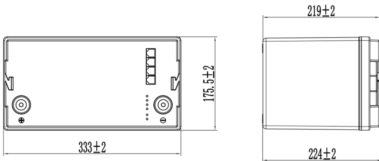
Figure 2-1 Picture of M12-150
