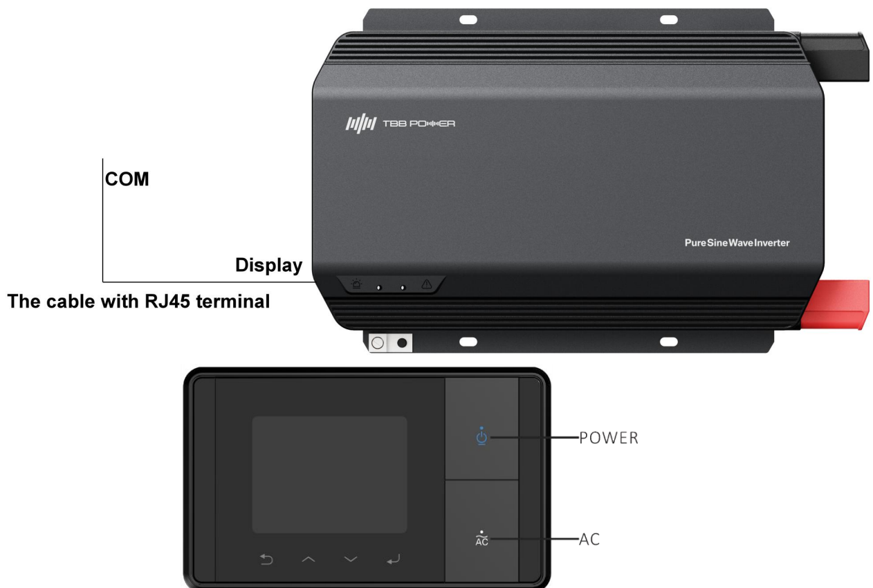
Figure 2-6 NH and VS28-LS Connection Diagram
