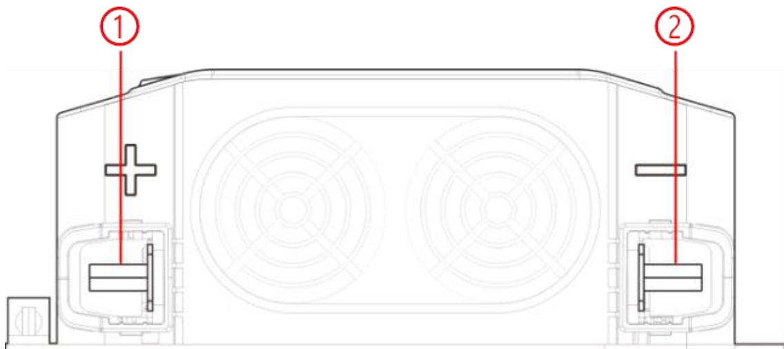
Figure 2-2 DC-side terminals diagram
