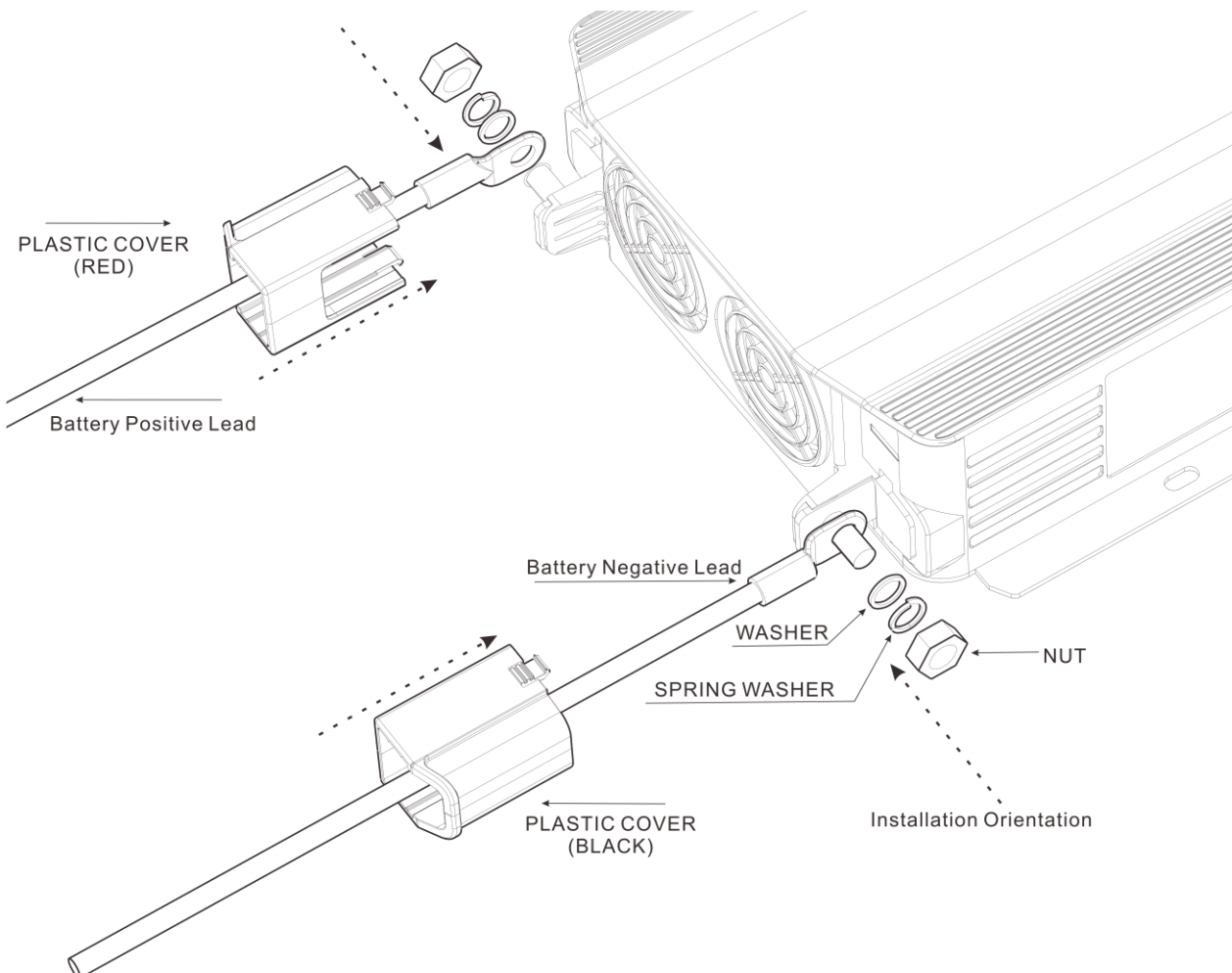
Figure 3-2 DC Cable Connection Diagram for NH
